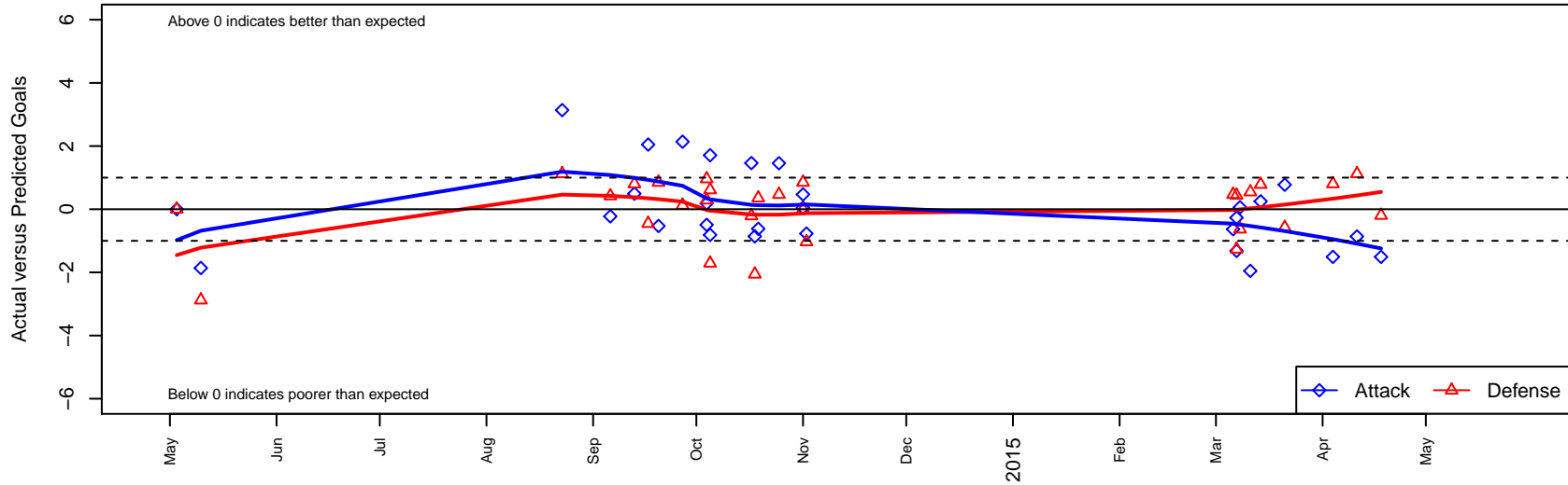
Boise Nationals Galaxy B01 Dots are actual minus expected GF (blue circles) and GA (red triangles). Blue line is smoothed change in attack strength. Red is smoothed change in defense strength.
